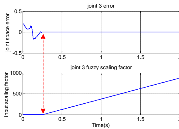
Figure 11. Scaling factor mechanism vs. joint3error in simulation A
