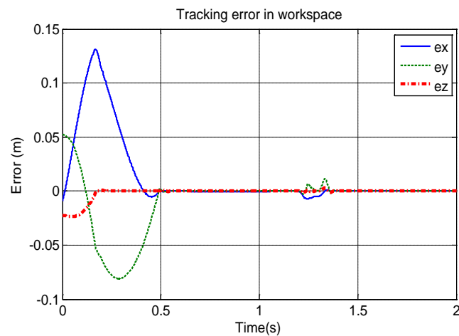
Figure 14. Work space tracking error in simulation B
