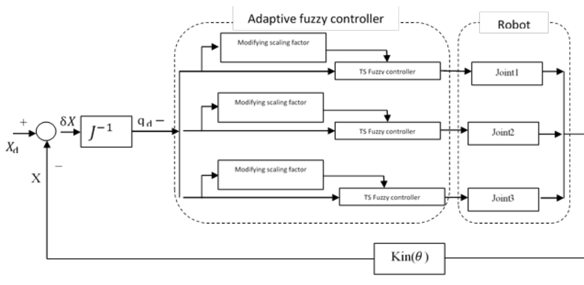
Figure 3. Control system
