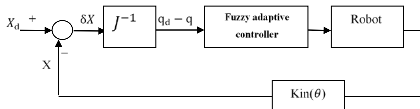
Figure 2. Inverse Jacobian strategy
