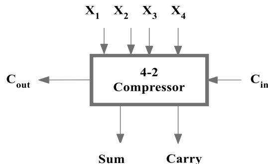
Figure 1. 4:2 compressors
