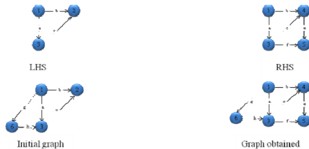
Figure 1. Basic concepts of graph transformation
